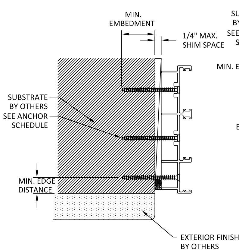
A 5 ANCHOR DETAIL THROUGH FRAME INSTALLATION
