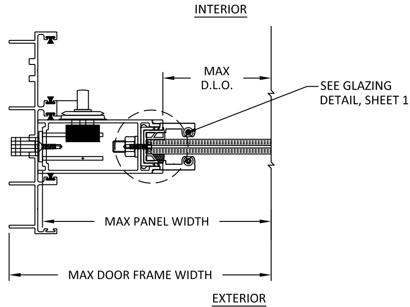
A 4 HORIZONTAL SECTION JAMB DETAIL
