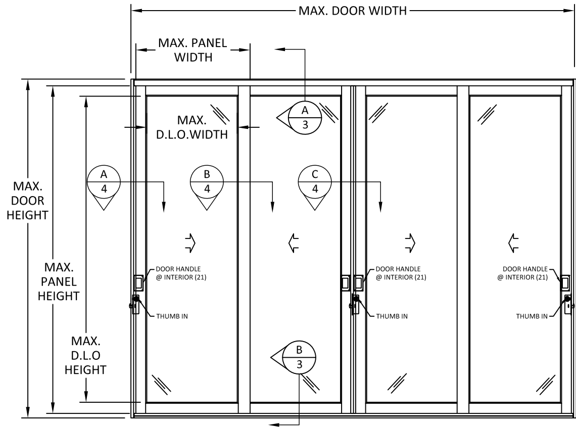
ELEVATION OUTSWING DOOR
