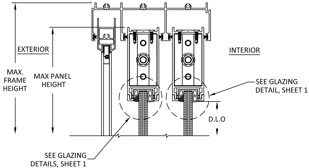
A 3 HORIZONTAL SECTION HEAD DETAIL
