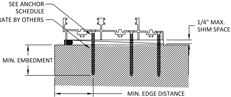
C 5 ANCHOR DETAIL THROUGH FRAME INSTALLATION
