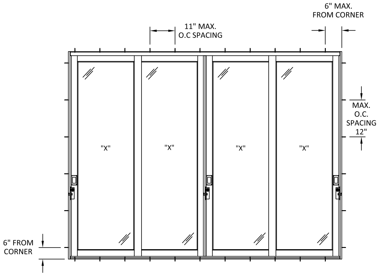
ANCHOR LAYOUT OUTSWING DOOR
